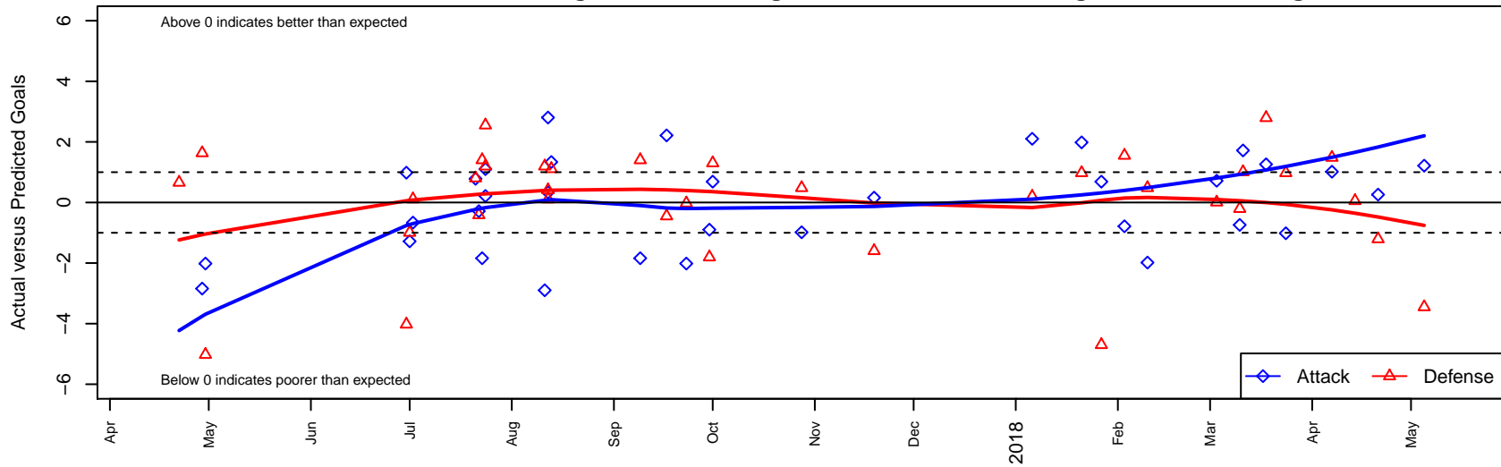
Crossfire Premier A B05 Dots are actual minus expected GF (blue circles) and GA (red triangles). Blue line is smoothed change in attack strength. Red is smoothed change in defense strength.
